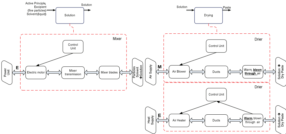
Figure 6. Exemplary Behaviors of the first two elementary functions of figure 4 represented through the TRIZ minimal model of a technical system.
