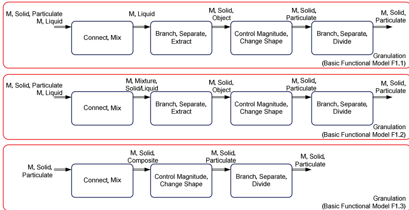
Figure 5. Elementary functions of the granulation phase according to the functional basis [18].
