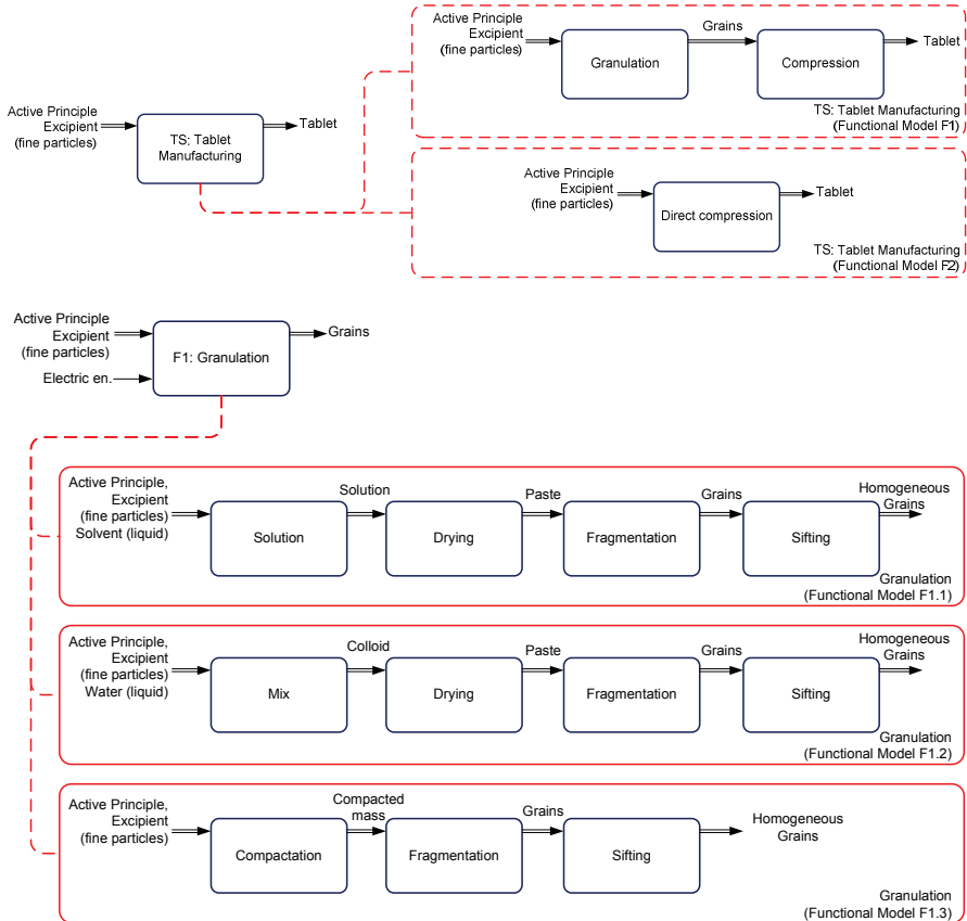
Figure 4. Functional model of a pharmaceutical tablet manufacturing process. EMS model of the overall TS and preliminary identification of the alternative technologies (above). Detailed functional decomposition of the granulation phase (below).
